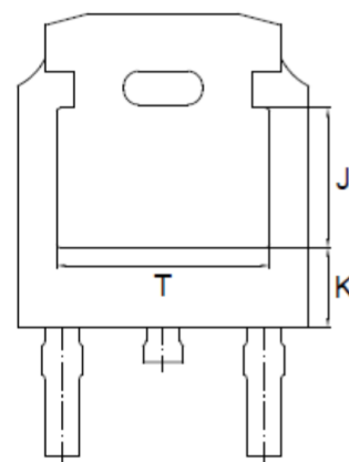
TO-252(D-PAK) mechanical data
