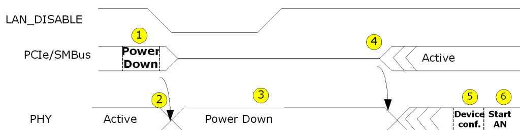
Figure 6. Power-Down Sequence
