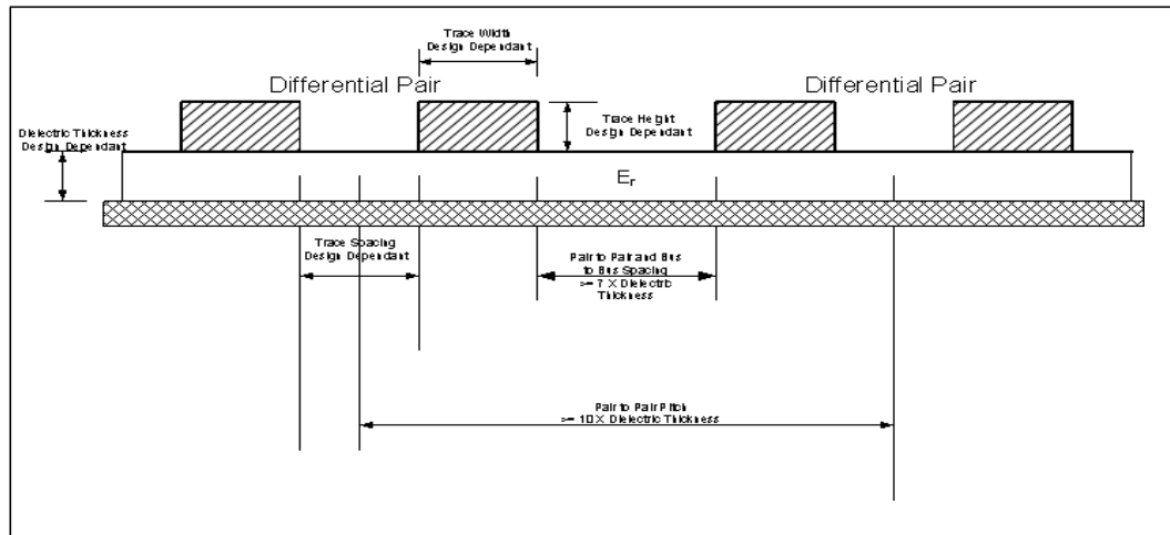
Figure 38. MDI Trace Geometry
