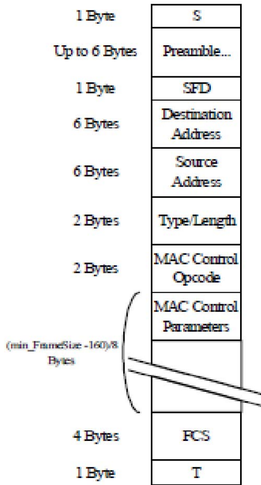
Figure 8. 802.3x MAC Control Frame Format
