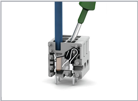
Insert fine-stranded conductors and remove all conductor types via operating tool.
