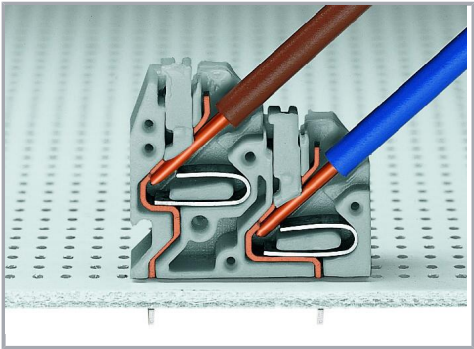
Space-saving wiring – push-in termination of solid conductors.
