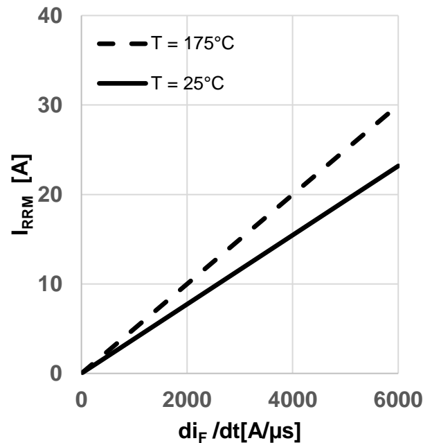
Figure 20 Typical reverse recovery current as a function of diode current slope ( I_{rrm} = f(di_i/dt) , V_{DD} = 800V , V_{GS} = 0V/18V , I_D = 16A , ind. load, test circuit in Fig.E, body diode at V_{GS} = 0V )
