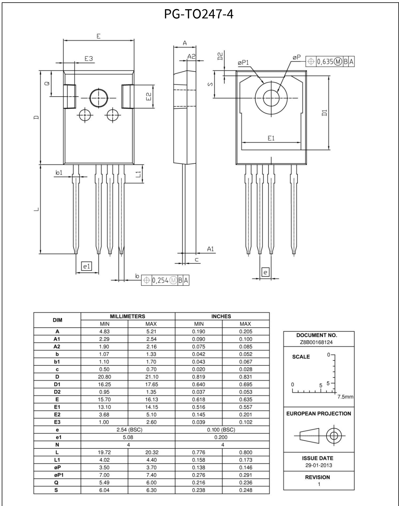
Figure 22 Package drawing
