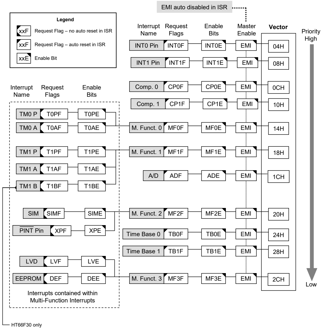
中断结构 – HT66F20/HT66F30
