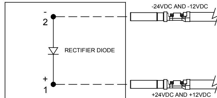
CONNECTOR DIAGRAM
