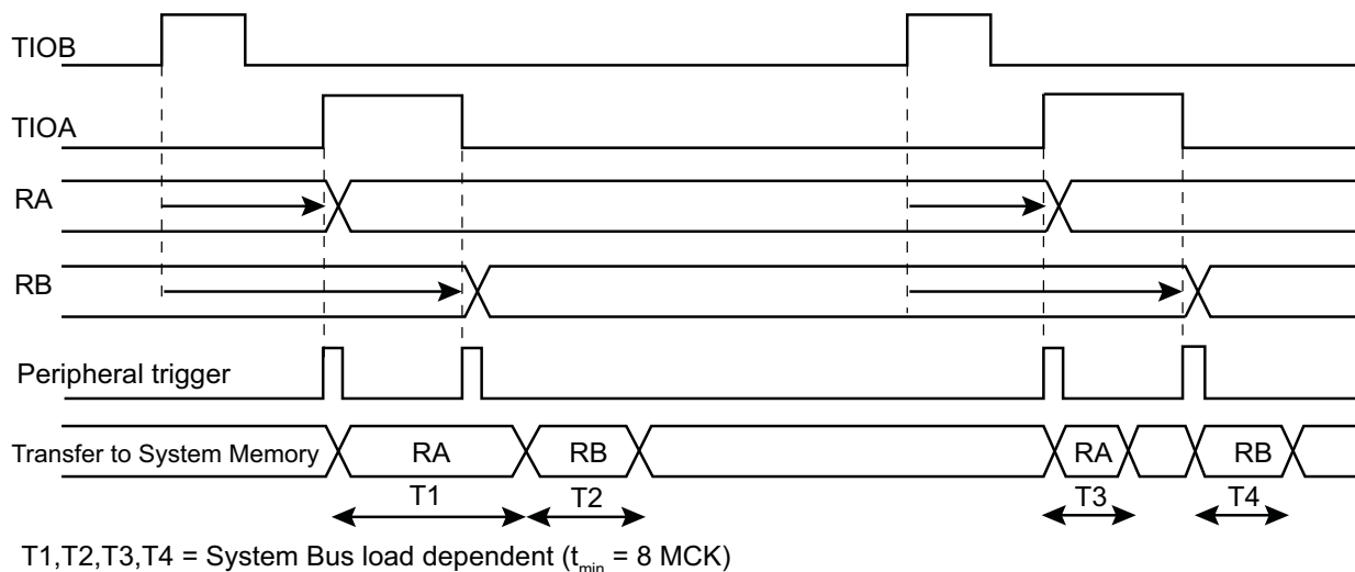
Figure 47-5. Example of Transfer with DMAC
