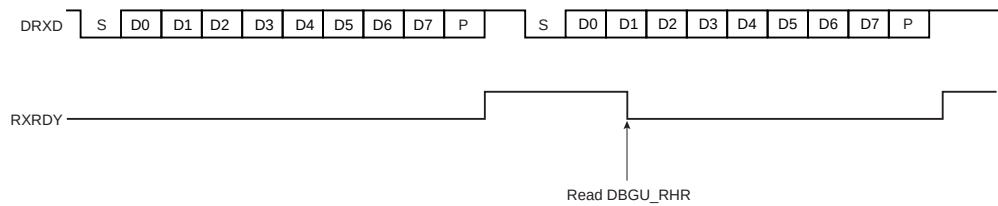
Figure 42-6. Receiver Ready
