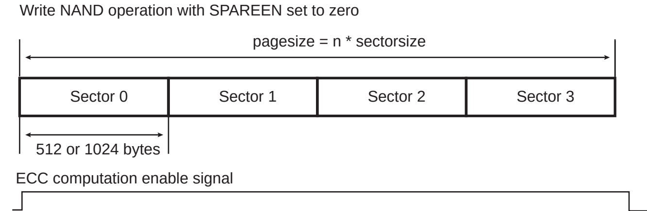
Figure 30-41.NAND Write Operation
