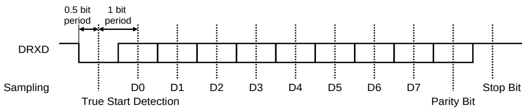
Figure 42-5. Character Reception
