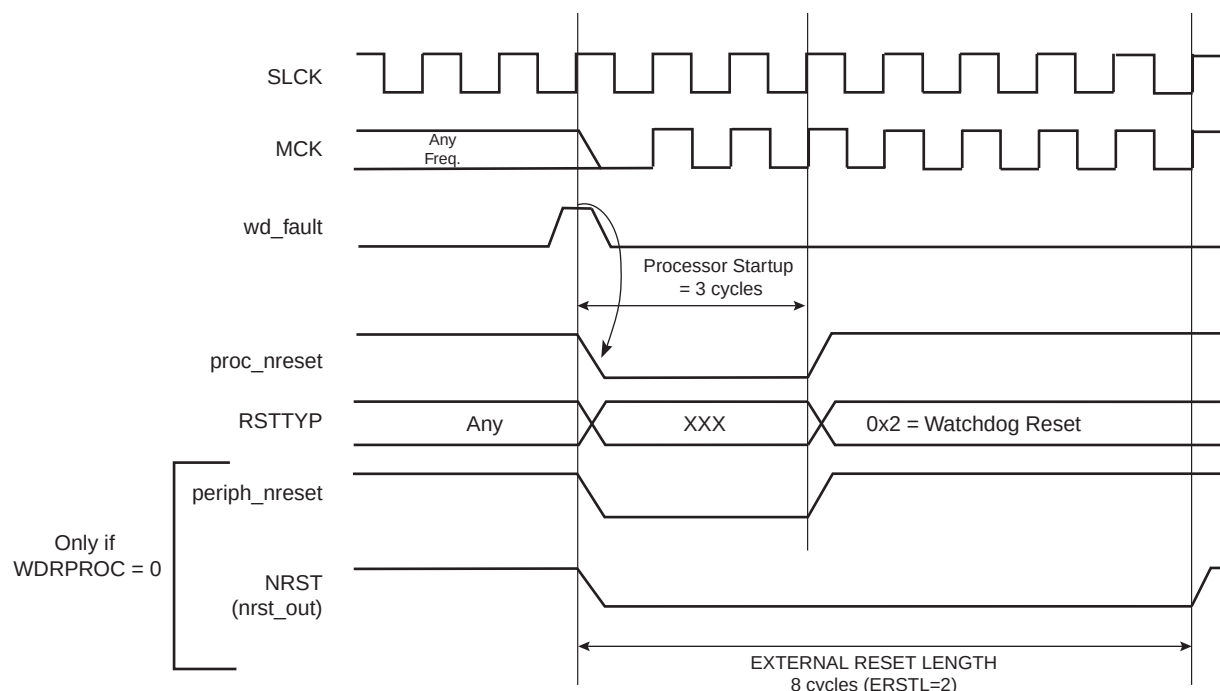
Figure 19-8. Watchdog Reset
