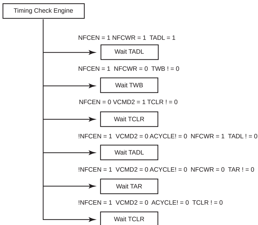
Figure 30-36.NAND Flash Controller Timing Engine
