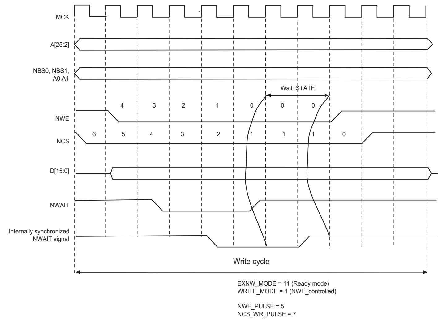
Figure 30-25.NWAIT Assertion in Write Access: Ready Mode (EXNW_MODE = 11)
