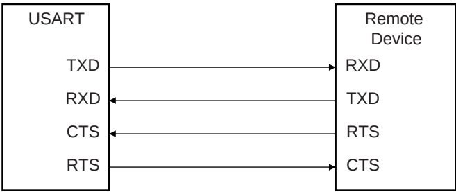
Figure 44-27.Connection with a Remote Device for Hardware Handshaking
