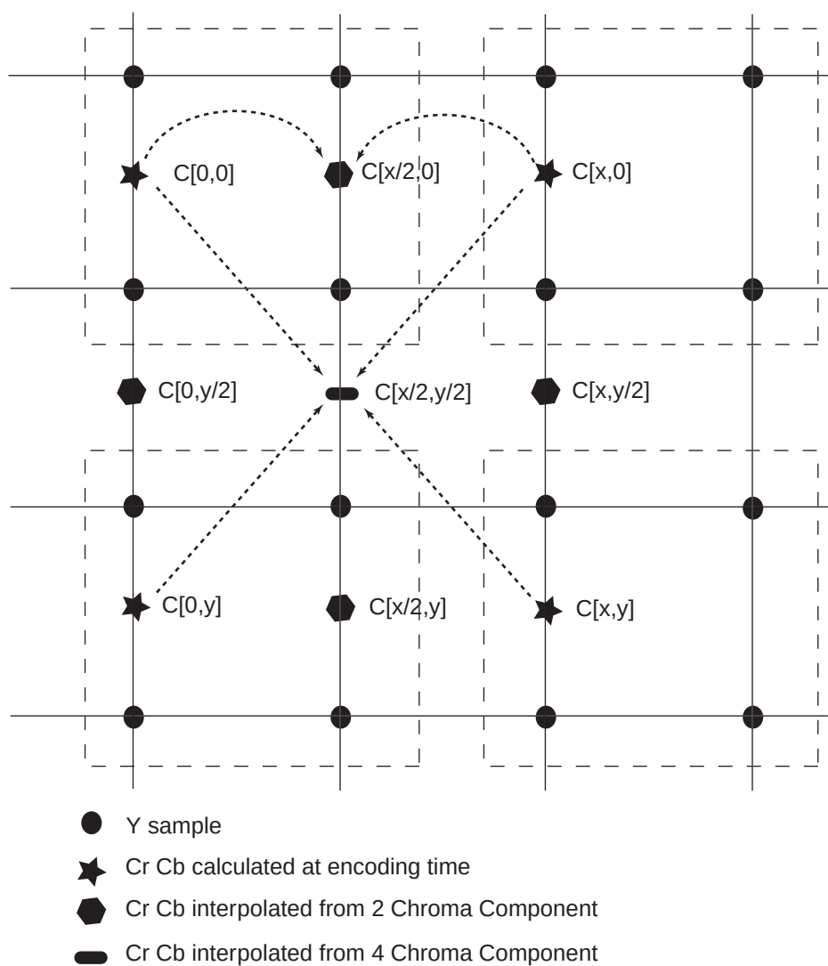
Figure 32-5. 4:2:0 Upsampling Algorithm
