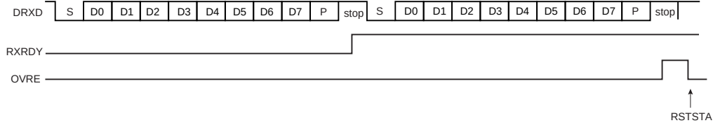
Figure 42-7. Receiver Overrun
