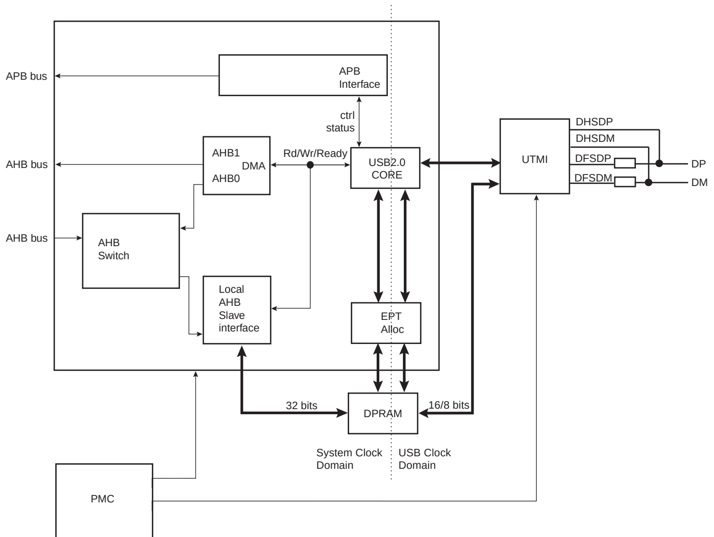
Figure 34-1. Block Diagram
