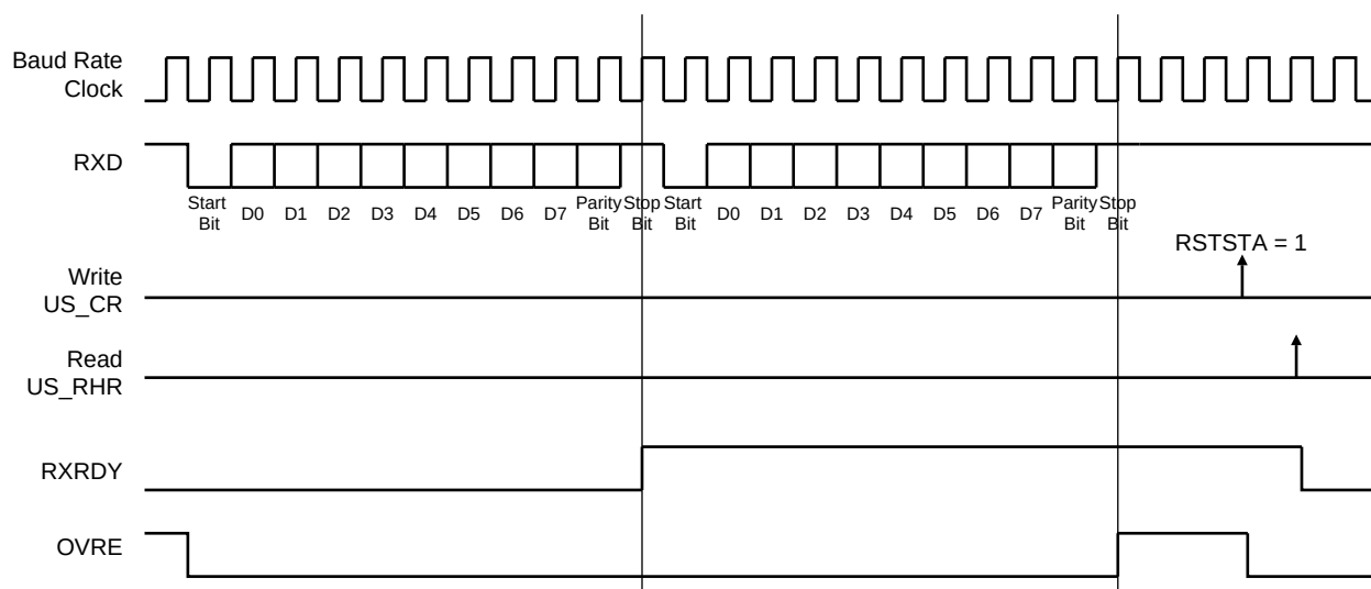
Figure 44-21. Receiver Status
