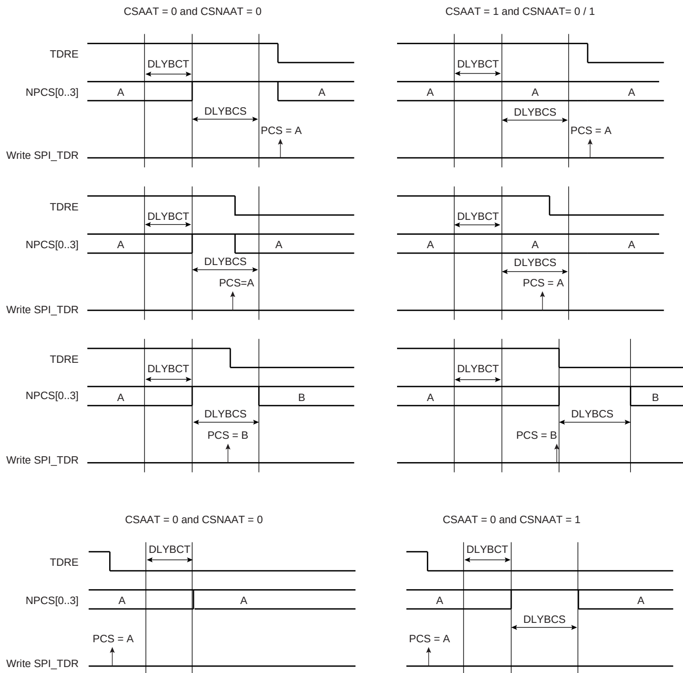
Figure 39-10. Peripheral Deselection
