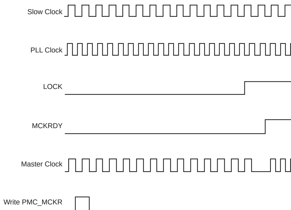
Figure 26-9. Switch Master Clock from Slow Clock to PLL Clock
