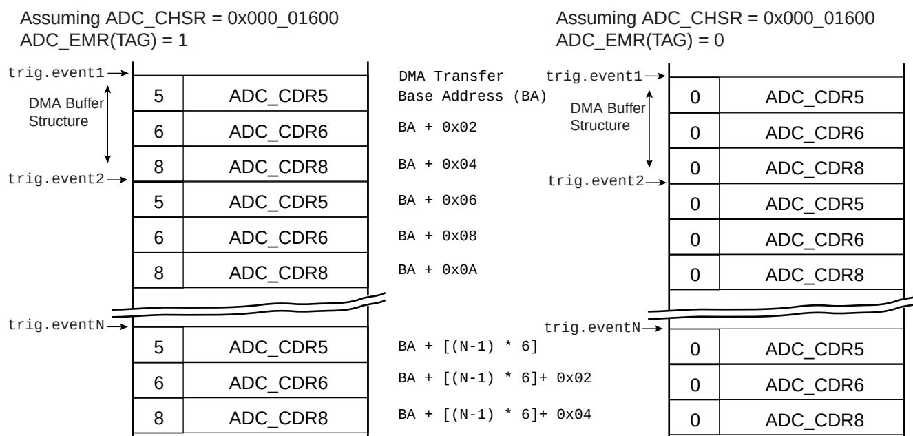
Figure 49-15. Buffer Structure when TSMODE = 0
