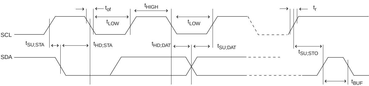
Figure 54-32. Two-wire Serial Bus Timing
