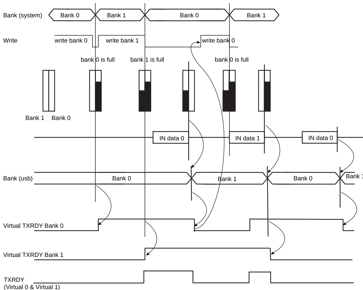
Figure 34-13.Autovalid with DMA
