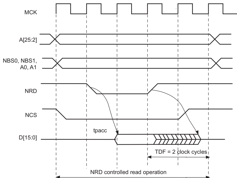
Figure 30-17.TDF Period in NRD Controlled Read Access (TDF = 2)
