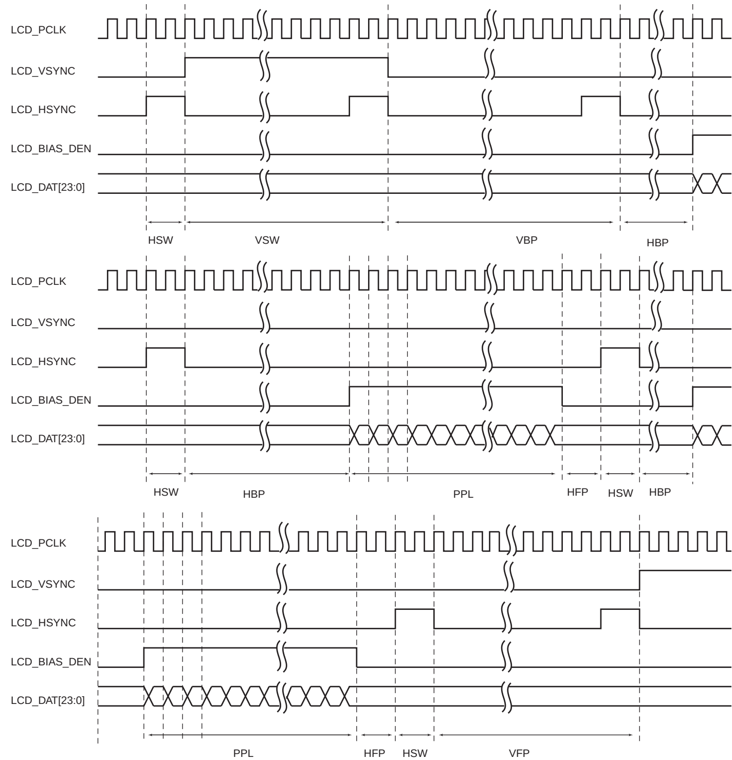
Figure 32-15.Active Display Timing
