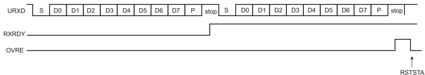
Figure 43-6. Receiver Overrun
