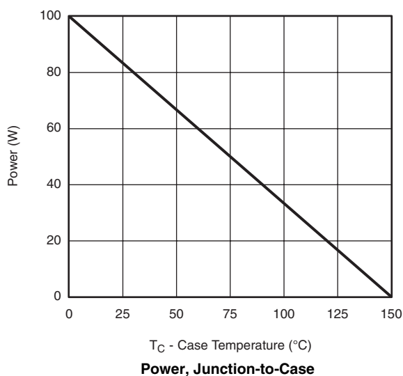
Power, Junction-to-Case
