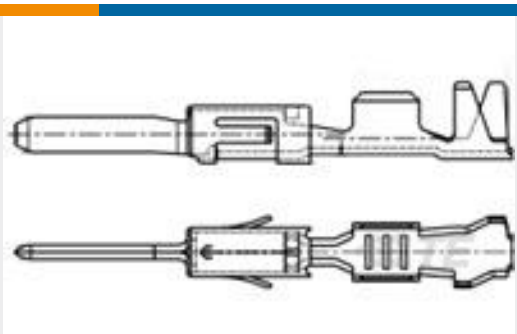
TE Part #963898-2 TAB A 1.6x0.6 CONTACT CF SRC Sn
