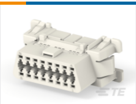
TE Part #2301724-5 16POS,060 SERIES,REC HSG,UNSLD
