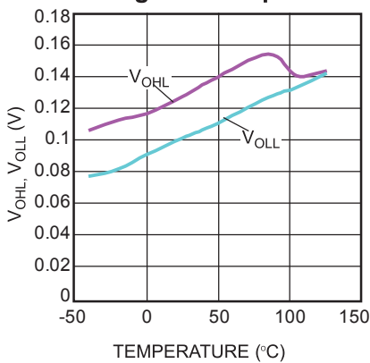
Low-Level Output Voltage vs. Temperature
