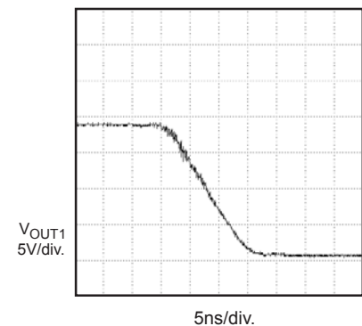
Output Fall-Time
