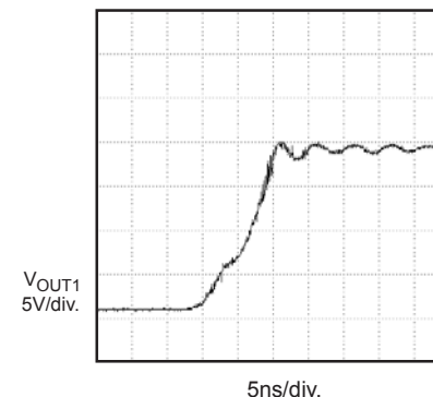
Output Rise-Time
