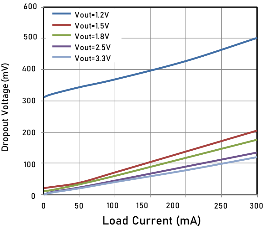
Dropout Voltage vs. Load Current
