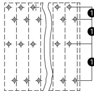
Dimensions in mm (1) Solder pins for deck 2 and 4 staggered by half the pin spacing
