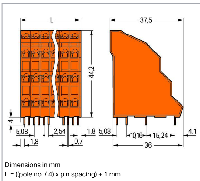
Dimensions in mm (1) Solder pins for deck 2 and 4 staggered by half the pin spacing
