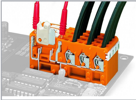
Distributing potentials via 3-conductor terminal blocks.
