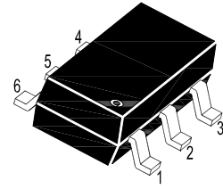
1.Anode 2. Anode 3.Anode 4. Cathode 5. Cathode 6.Cathode SOT-363 Plastic package Marking Code : KA
