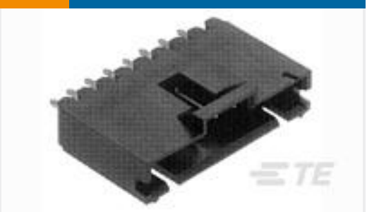
TE Part #6-103639-3 14 MTE HDR SRST LATCH .100CL
