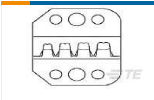
TE Part #2063530-2 SDE MQS 0.5-0.75mm2 DIE SET
