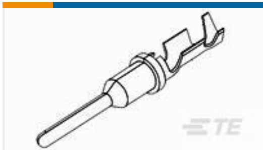
TE Part #776300-1 PIN CONTACT WIRE TO WIRE LOOSE
