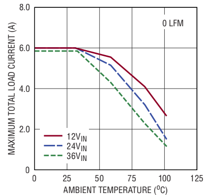
Derating, V_{OUT} = 8\text{V} BIAS = 5V, DC2860A Demo Board T_J = 120^\circ\text{C} , Burst Mode All Channels At Same Load
