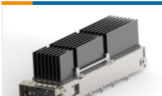
TE Part #2342933-3 QSFP-DD 1X1, STANDARD, W/ EXTRUDED HS
