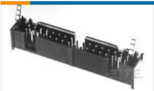
TE Part #1761606-7 IDC LOW PRO HDR 20P VERT LG LAT BLK
