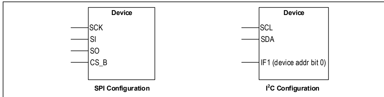
FIGURE 7-1: Host Interface Pins for SPI and I 2 C.
