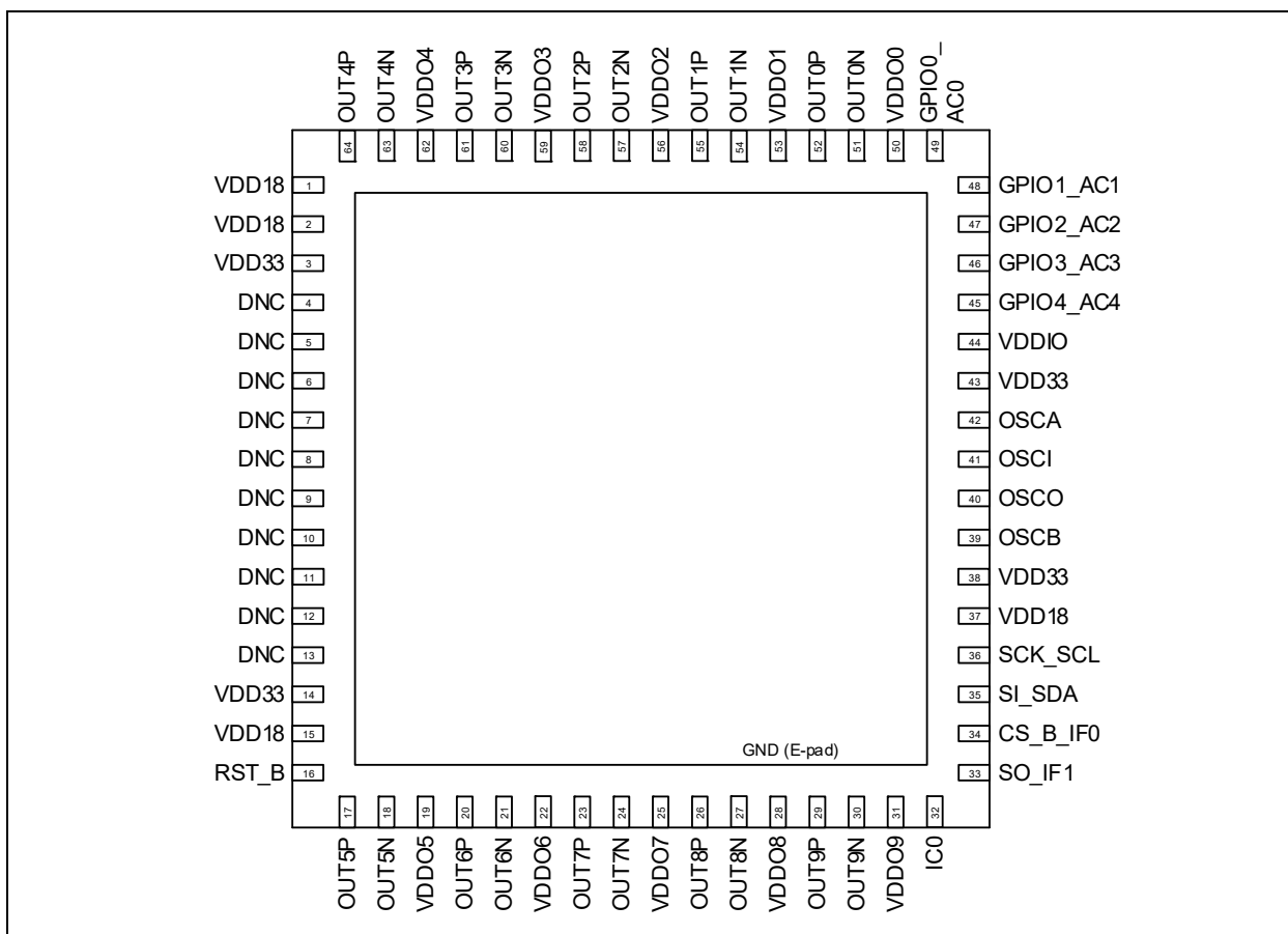
FIGURE 3-1: 64-Lead 9 mm x 9 mm VQFN (0.5 mm pitch) for ZL30271.
