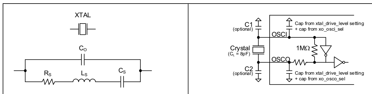
FIGURE 5-2: Crystal Equivalent Circuit/Recommended Crystal Circuit.
