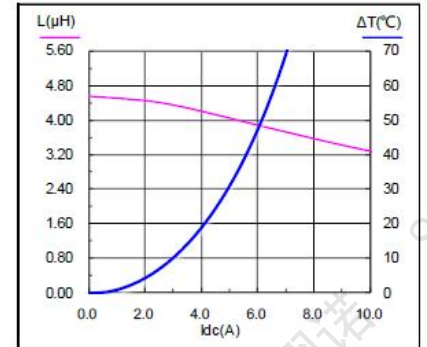
SMMS0630-4R7M
