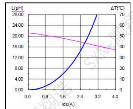
SMMS0630-220M
