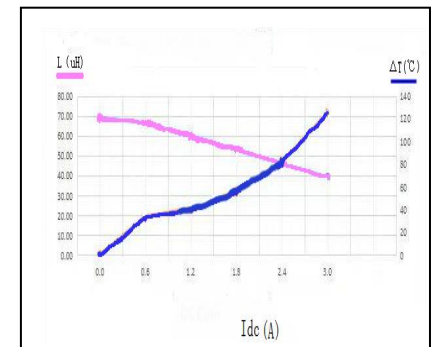
SMMS0630-680M
