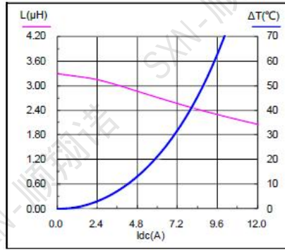
SMMS0630-3R3M
