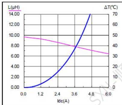
SMMS0630-100M
