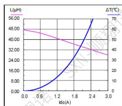
SMMS0630-470M
