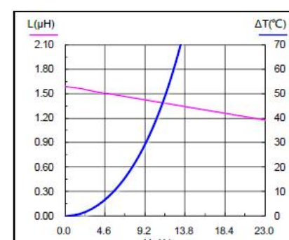
SMMS0630-1R5M
