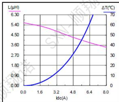
SMMS0630-5R6M
