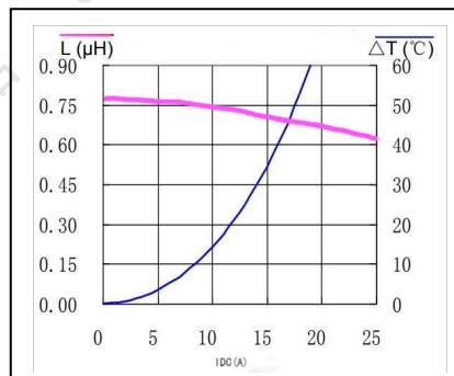
SMMS0630-R82M
