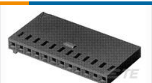
TE Part #102241-2 04 MODIV HG COMP SR .100 POL
