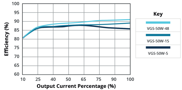
EFFICIENCY VS OUTPUT LOAD (at 230 Vac)
