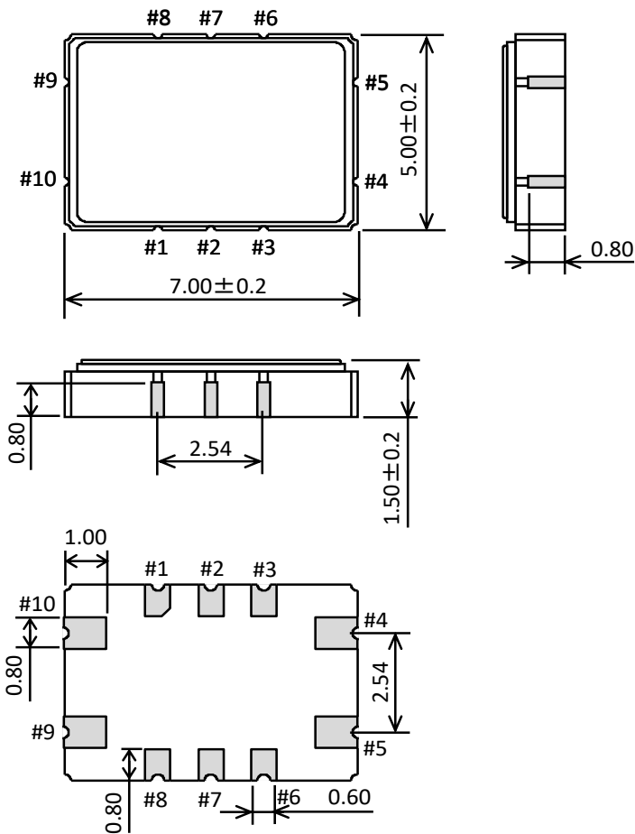
[ 8 ] Outline Drawing unit: mm
