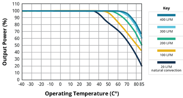
TEMPERATURE DERATING CURVE PRQ150W-Q48-S24-D (Baseplate version) ( V_{in} = 24\text{ V} )
