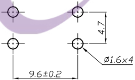
PCB MOUNTING HOLE ARRANGEMENT
