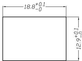
PANEL CUTOUT DIMENSION:
