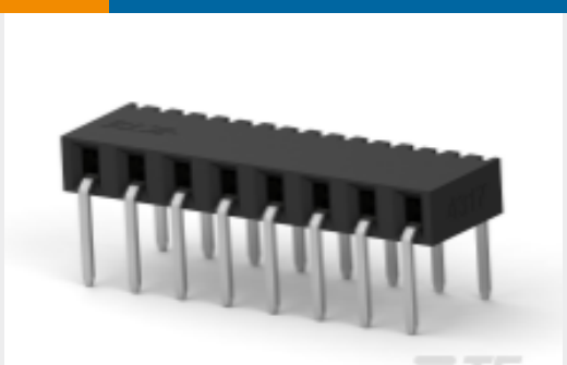
TE Part #2314928-8 8P,2MM,B-B,REC,SRHZ,2.1,0.1AU,TB
