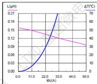
SMS0630-R15M
