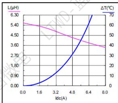
SMS0630-5R6M
