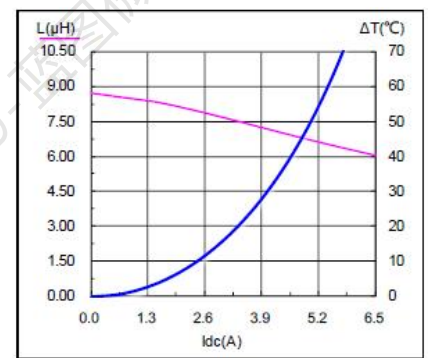
SMS0630-8R2M
