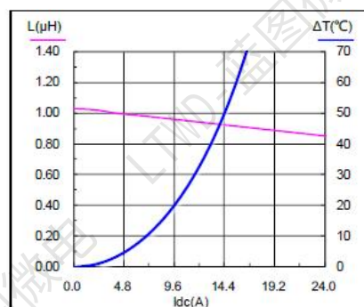
SMS0630-1R0M
