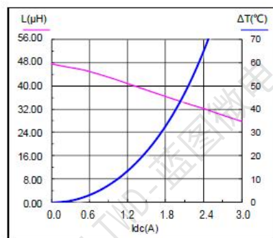
SMS0630-470M
