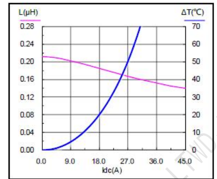
SMS0630-R22M
