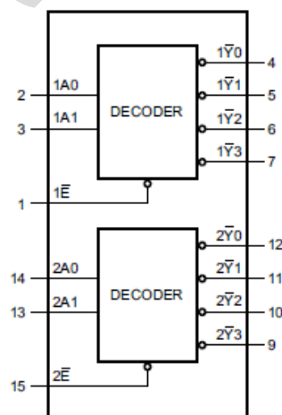
Figure 3. Functional diagram
