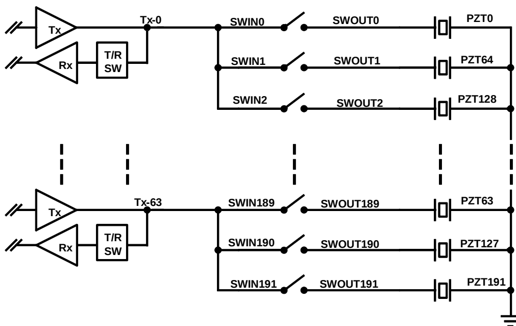
Figure 18: Typical Application Circuit
