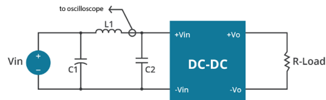
Figure 1 Measuring Input Ripple Current
