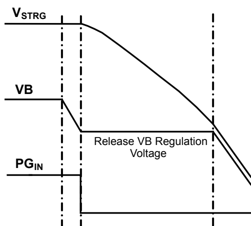
Figure 4: Release Times
