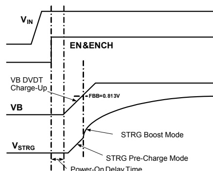
Figure 2: Charging Process
