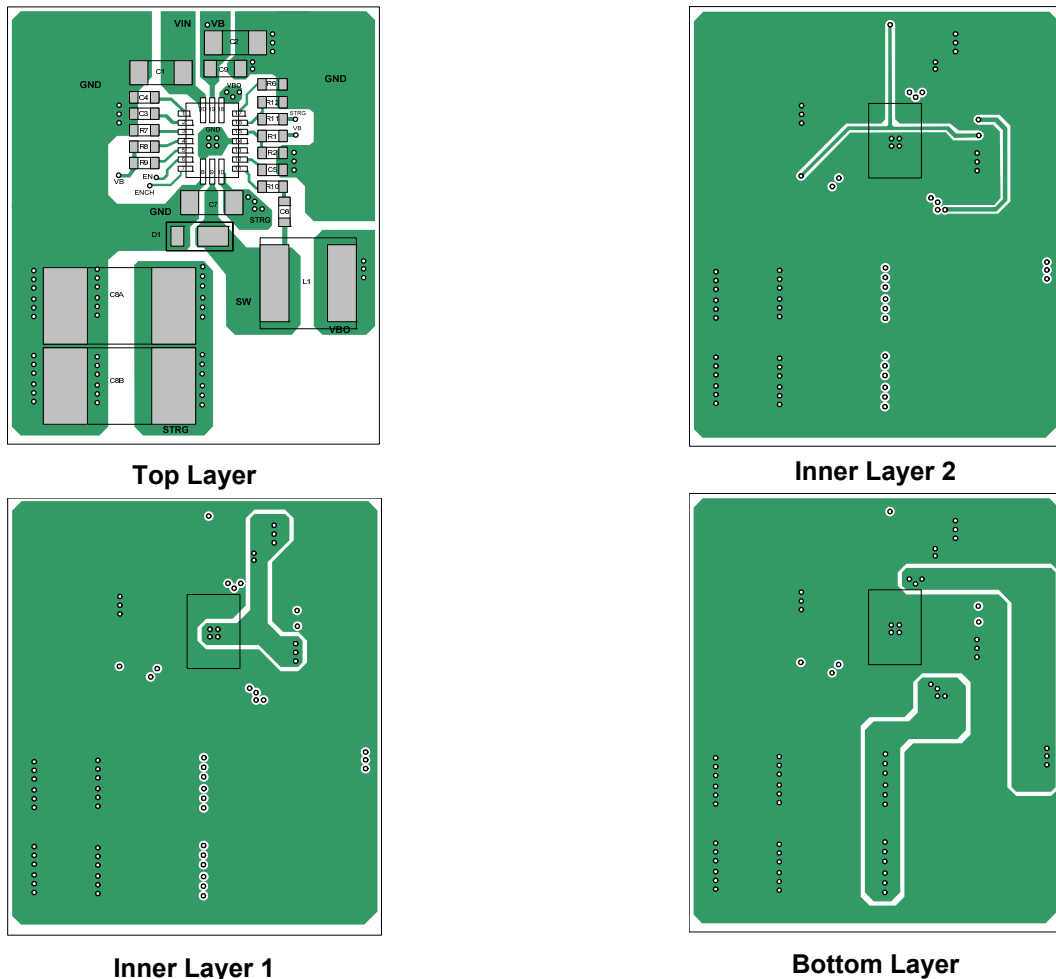
Figure 7: Recommended Layout
