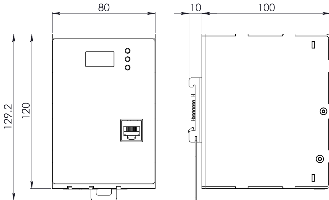
Figure 2. Mechanical Drawing
