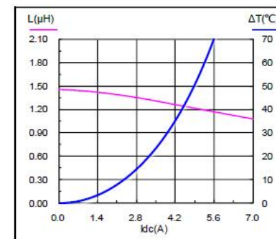
SMS0420-1R5M
