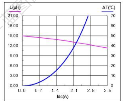
SMS0420-150M
