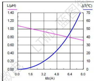
SMS0420-1R2M
