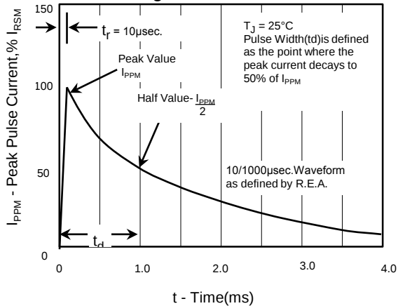
Fig.3 - Pulse Waveform
