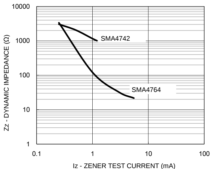
Fig.3 Typical Zener Impedance
