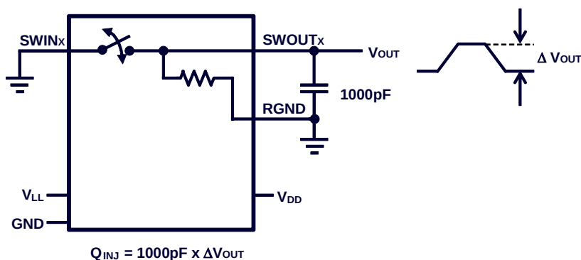
Figure 9: Test Circuit 8
