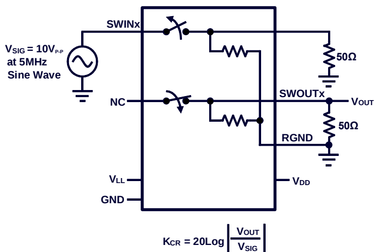
Figure 7: Test Circuit 6
