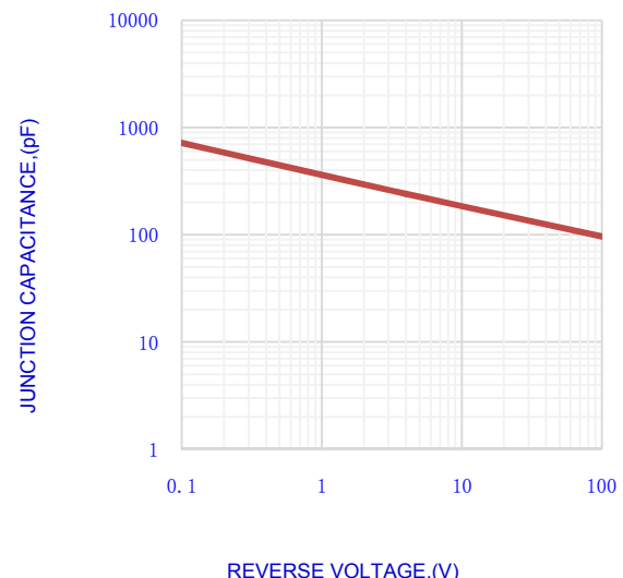
Fig.4-TYPICAL JUNCTION CAPACITANCE
