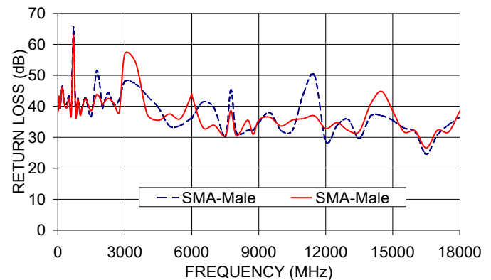
141-24SM+ RETURN LOSS
