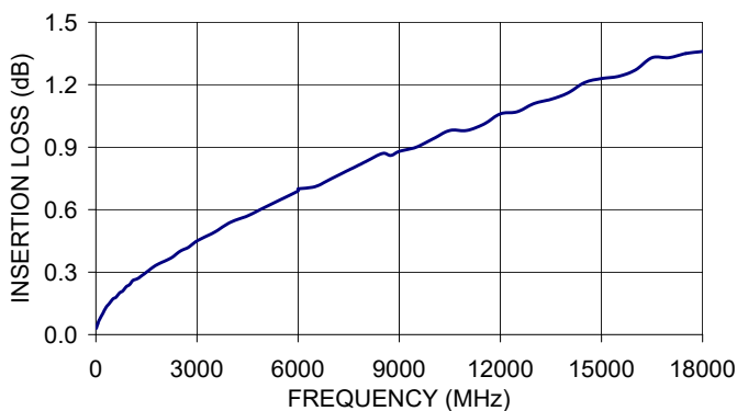
141-24SM+ INSERTION LOSS
