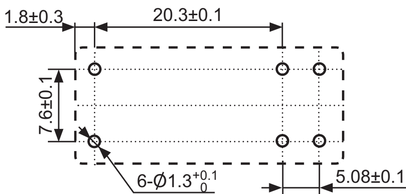
Recommended PCB Layout Bottom View
