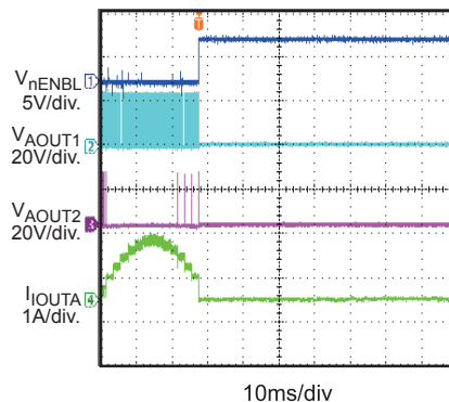
Disable-Eighth Step
