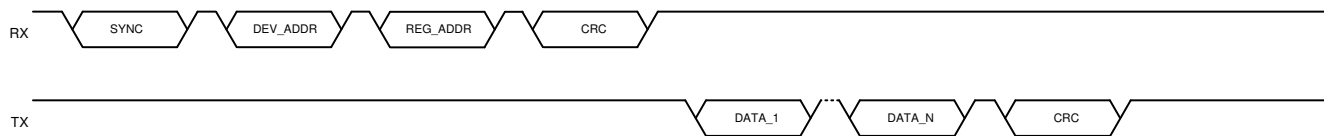
Figure 7-19. Multiple Data Bytes Read in Burst Mode
