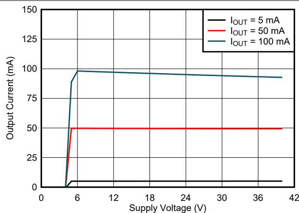
Figure 6-5. Output Current vs Supply Voltage
