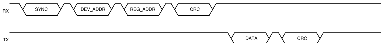
Figure 7-14. Single-Byte Readback Command
