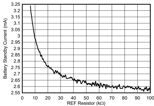
Figure 6-1. Standby Current vs REF Resistor
