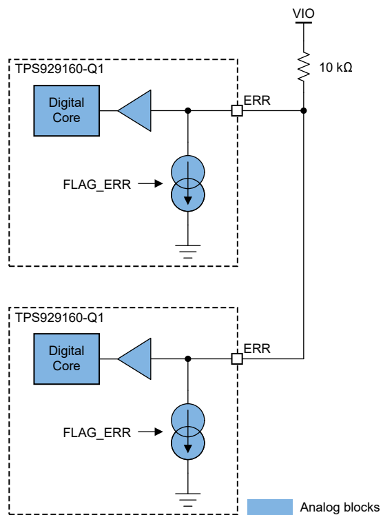
Figure 7-10. ERR Internal Block Diagram
