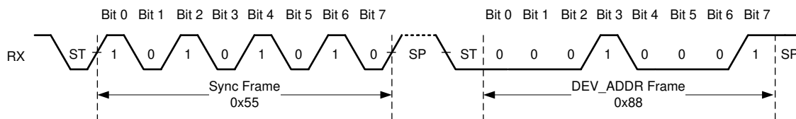
Figure 7-15. Synchronization Byte
