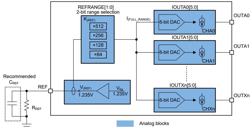
Figure 7-1. Output Current Setting
