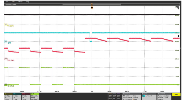
Figure 6-25. LED Open-Circuit Detection in Normal Mode
