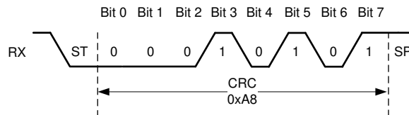
Figure 7-17. CRC Byte
