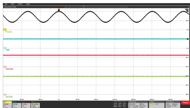
Figure 6-18. Transient Overvoltage
