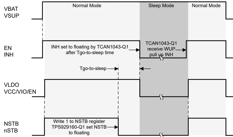
Figure 7-8. Sleep Mode Access and Exit Timing Diagram
