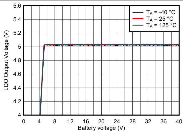
Figure 6-8. LDO Output Line Regulation
