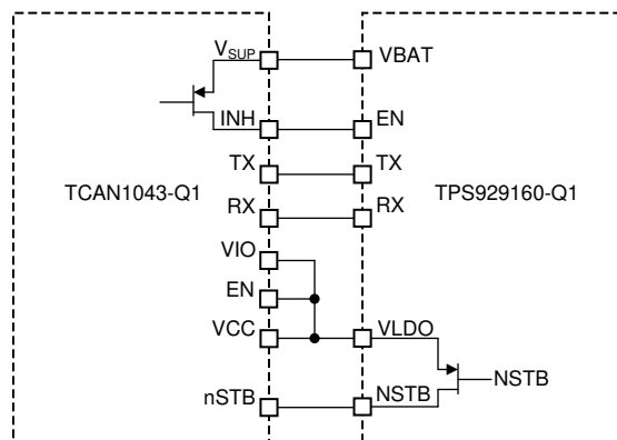
Figure 7-7. Sleep Mode Typical Application Diagram
