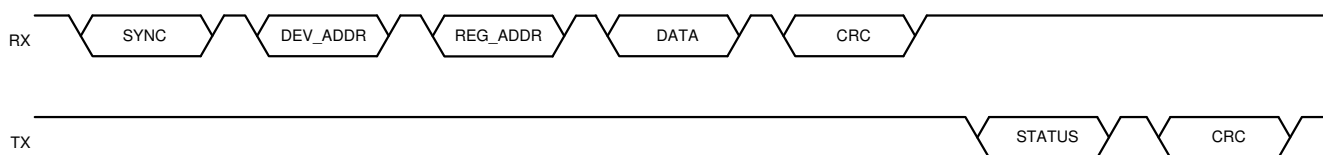
Figure 7-13. Single-Byte Write Command with Status Feedback
