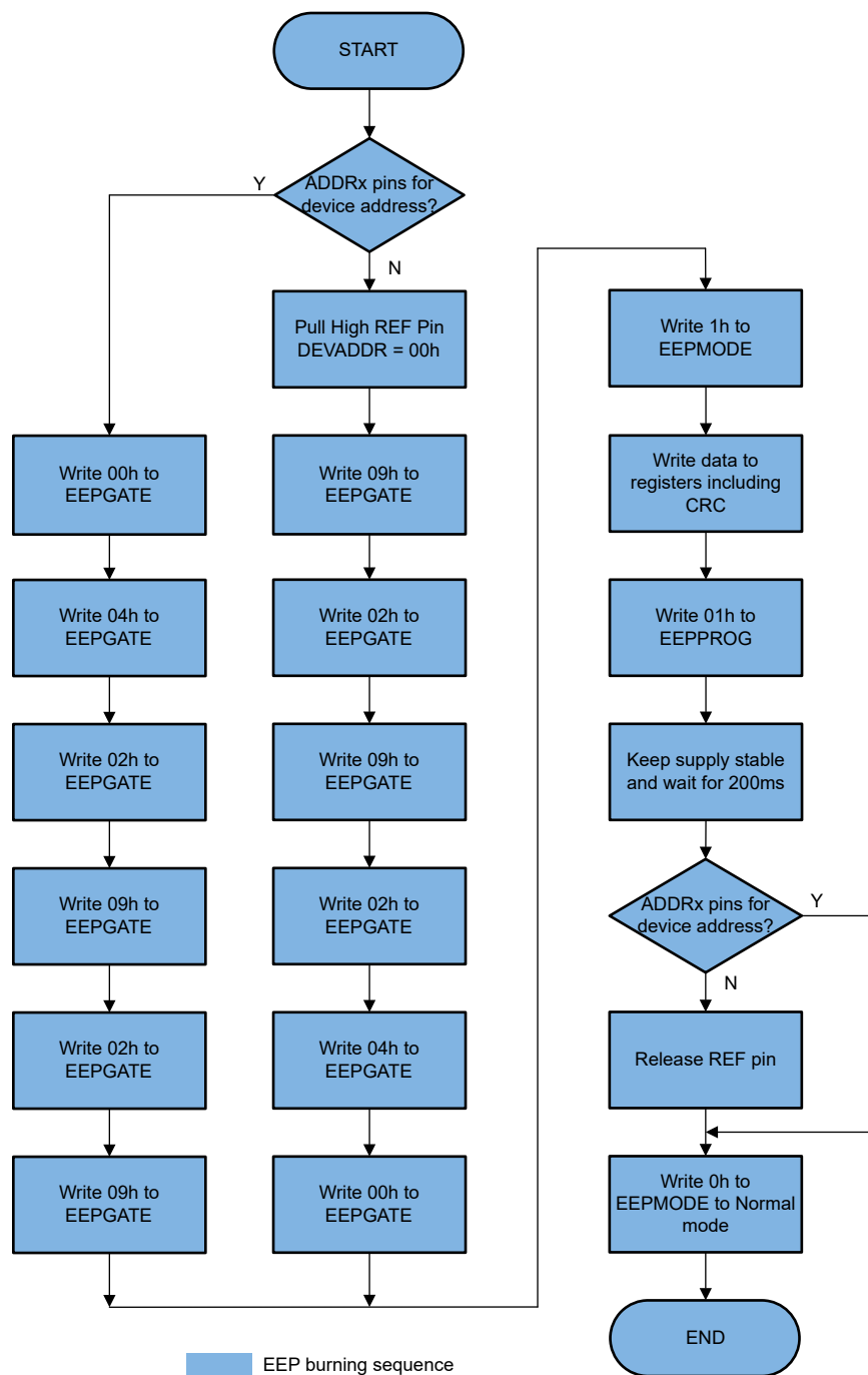
Figure 7-20. Programming Sequence
