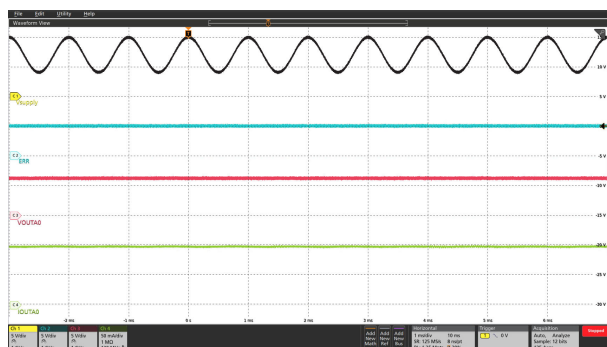
Figure 6-19. Jump Start
