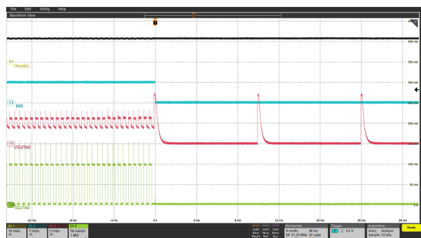
Figure 6-26. LED Short-Circuit Detection in Normal Mode
