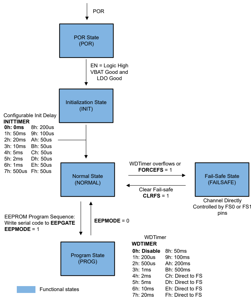
Figure 7-11. Device Functional Mode State Machine
