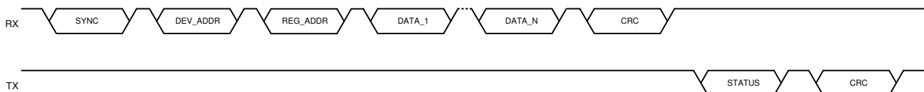
Figure 7-18. Multiple Data Bytes Write in Burst Mode
