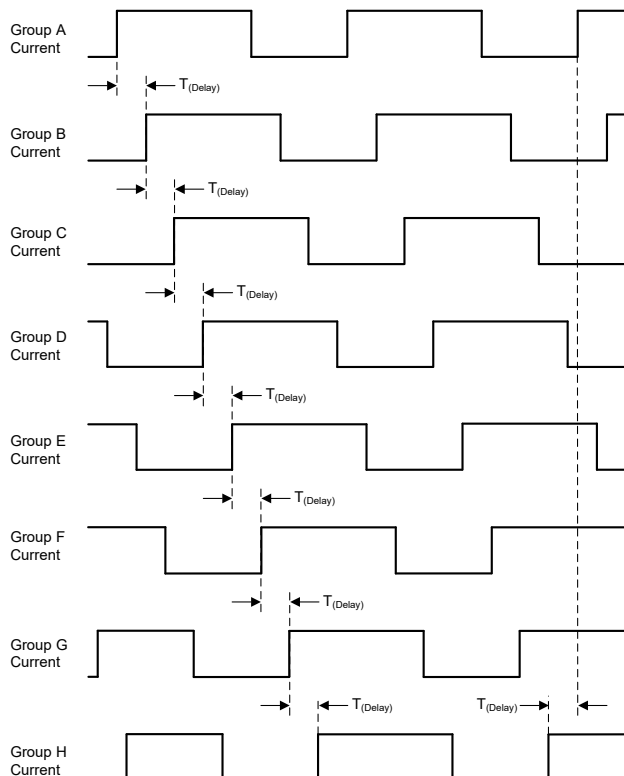
Figure 7-4. Phase Shift Dimming Mode
