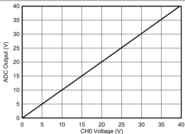
Figure 6-11. ADC sampling result vs sampled channel voltage
