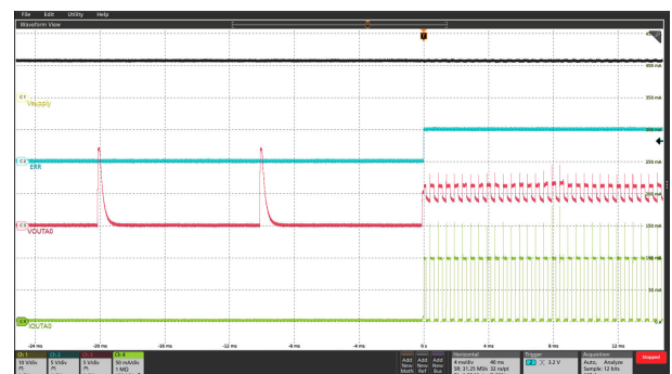
Figure 6-27. Single-LED Short-Circuit Detection in Normal Mode
