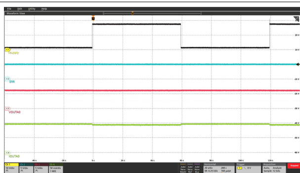
Figure 6-19. Jump Start
