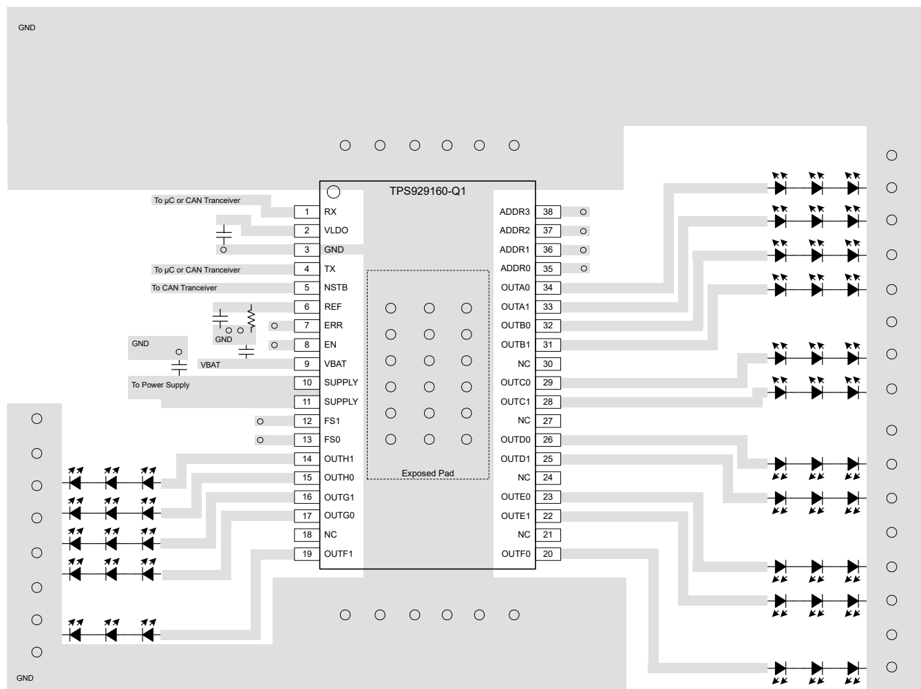
Figure 8-5. TPS929160-Q1 Layout
