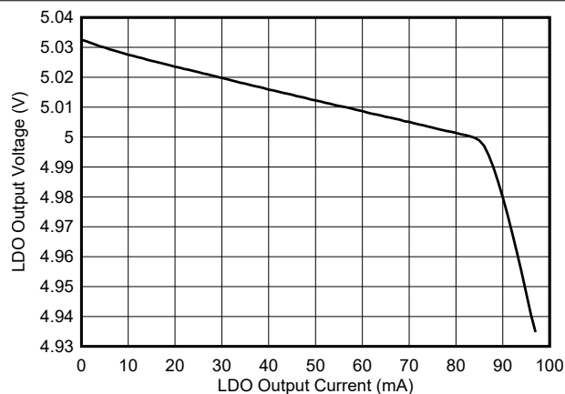
Figure 6-9. LDO Output Load Regulation
