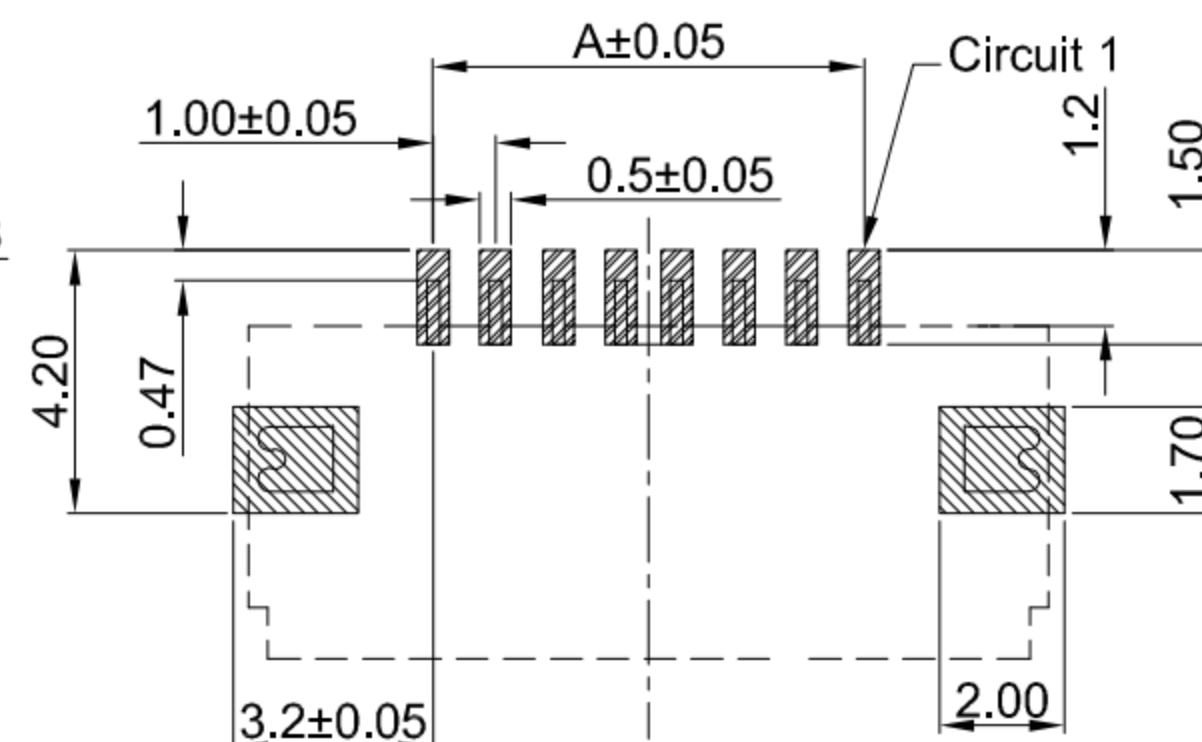
RECOMMENDED PCB LAYOUT TOLERANCE: \pm 0.05
