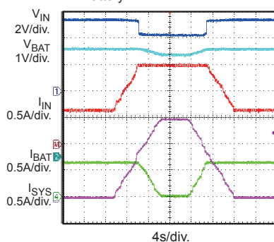
Power Path Management MODE=1, 1.5A Source Current Limit, W/ Battery
