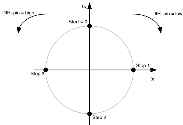
Figure 14. Full-Step 1/2 Rotated
