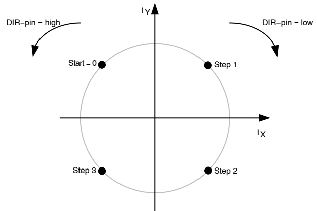
Figure 15. Full-step
