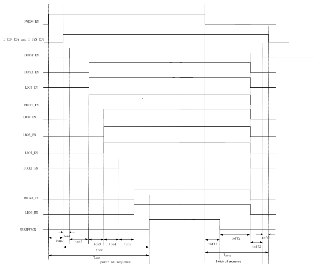
Fig. 4-3 Power On/Off Timing, BOOT1=0, BOOT0=1
